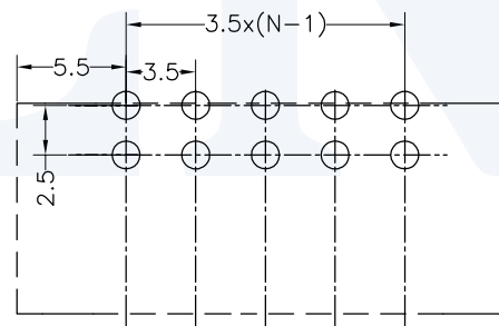
Recommended P.C.B Layout(Top Side)
