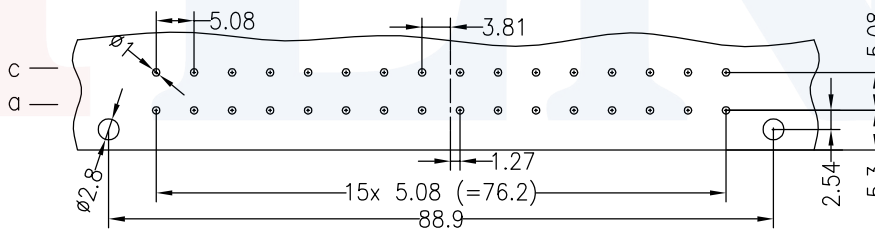
PCB LAYOUT(RECOMMENDED)
