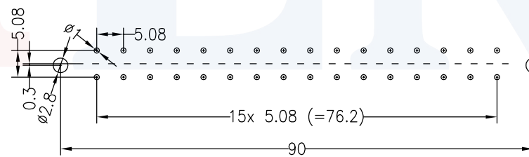
PCB LAYOUT(RECOMMENDED)
