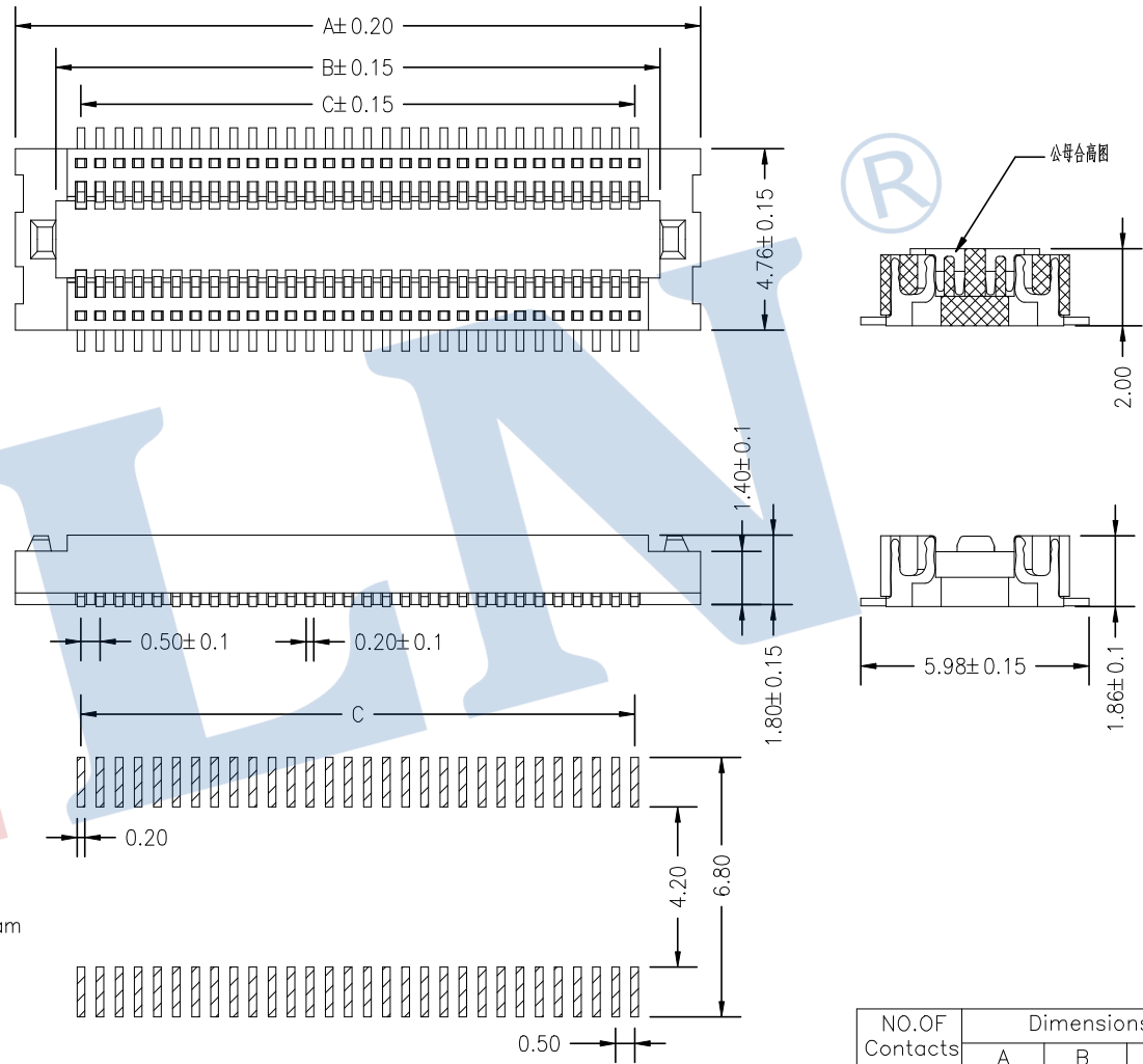
Recommended P.C.B Layout(Top Side) (PCB BOARD TOLERANCE±0.05)
