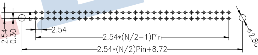
Recommended P.C.B Layout(Top Side) (PCB BOARD TOLERANCE±0.05)
